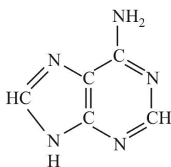
Adenine (A)
