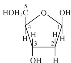
\beta -D-2-deoxyribose
