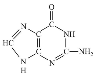
Guanine (G)
